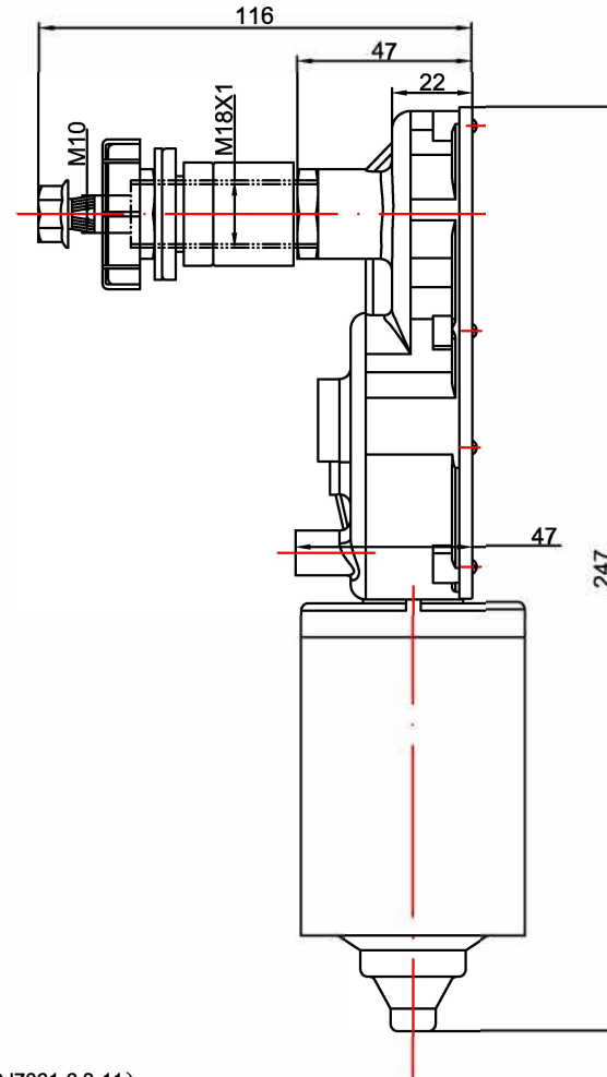
motor socket (model: DJ7061-6.3-11)
