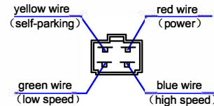
motor socket (model: DJ7061-6.3-11)
